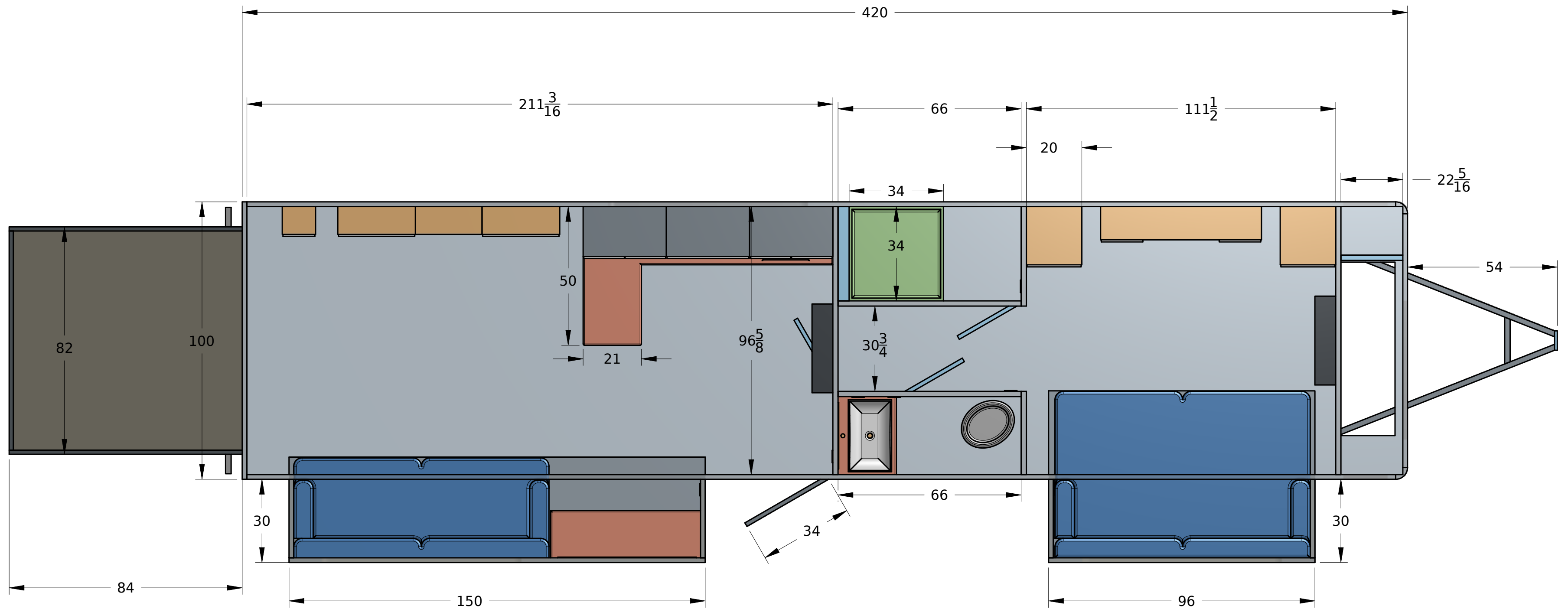
40' Single Cast Trailer W/Patio
